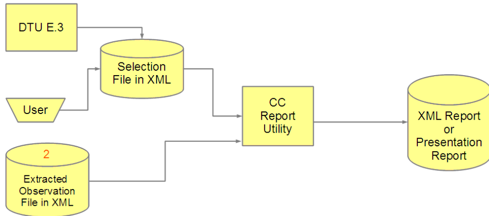
Figure 5. Step 3 Code coverage report process
